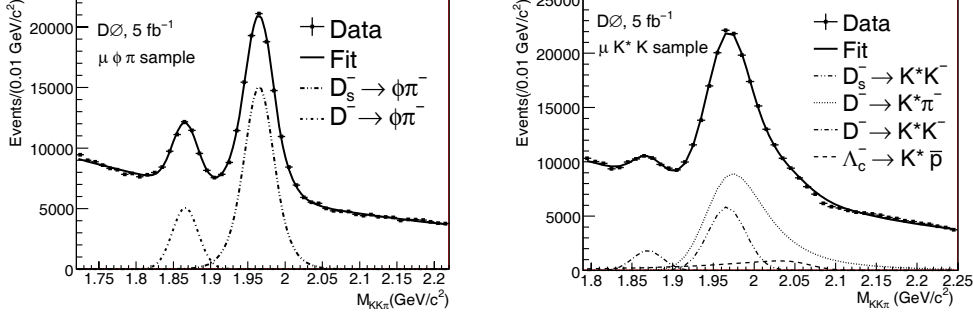
Fig. 2. – Mass distributions observed in the DØ a_{fs}^s analysis. The D_s^- \rightarrow \phi\pi^- channel can be seen in the left plot, the D_s^- \rightarrow \mu^+ K^{*0} K^- on the right.
