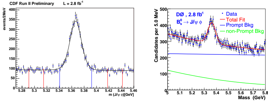
Fig. 3. – Mass distribution of the B_s^0 \rightarrow J/\psi \phi signal sample for the CDF (left) and the D0 analysis (right).
