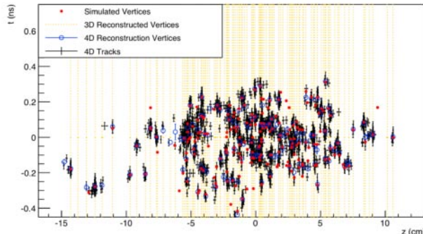
Fig. 1. – Comparison between 3D (vertical yellow lines) and 4D (blue open circles) reconstructed vertices in a bunch crossing with PU 200 [1]. Simulated vertices are marked by red dots. The black crosses represent tracks reconstructed including time information. The horizontal axis is the z -position along the beamline, while the vertical axis is the time.
