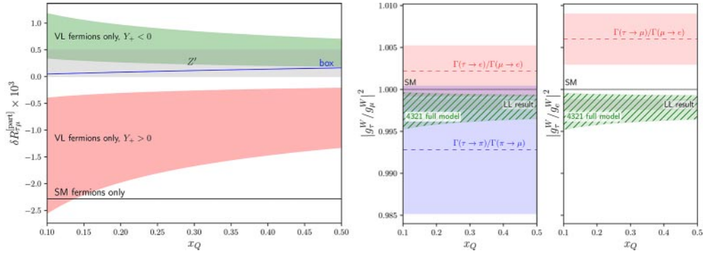
Fig. 2. – Numerical analysis of the modifications to leptonic decays. Left: different contributions to \delta R_{\tau\mu} as function of x_Q = m_Q^2/m_V^2 . The black line is the contribution from the box diagrams involving SM fermions only. The red and green bands summarize all contributions involving one or more vector-like quarks for Y_+ > 0 and Y_+ < 0 , respectively. The grey band is obtained varying s_\tau , while the blue line comes from the box diagram with two leptoquarks and four external leptons. Right: Comparison with current experimental determination of the 4321 prediction for two LFU ratios. Both the hatched and grey bands have been obtained varying C_U from 0.005 to 0.01, corresponding to the best-fit value to the B anomalies in the presence or absence of right-handed currents.
