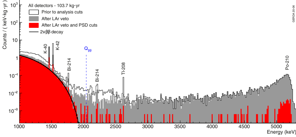
Fig. 2. – GERDA Phase II energy distribution (103.7 kg · yr of exposure) before and after the application of active background reduction techniques (LAr veto and PSD) [27]. The expected 2\nu\beta\beta decay spectrum is shown assuming the half-life of 1.93 \times 10^{21} yr measured by GERDA [28]. The \gamma -lines and the \alpha events around 5.3 MeV are also labeled.
