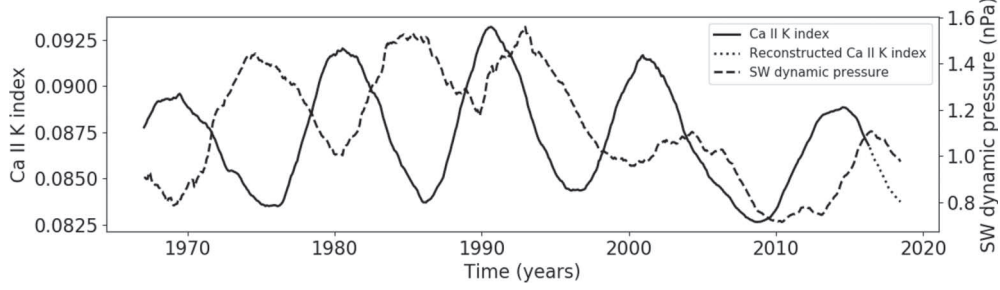
Fig. 1. – 37 month moving averages of the Ca II K index (continuous line) and solar wind dynamic pressure (dashed line). The dotted line shows the reconstructed Ca II K index obtained using the linear relation with the Mg II index.
