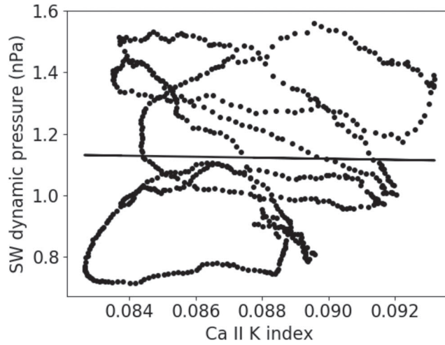
Fig. 2. – Relationship between 37 month moving averaged solar wind dynamic pressure and Ca II K index. The solid line shows the linear fit. The correlation coefficient is R = -0.0195 .
