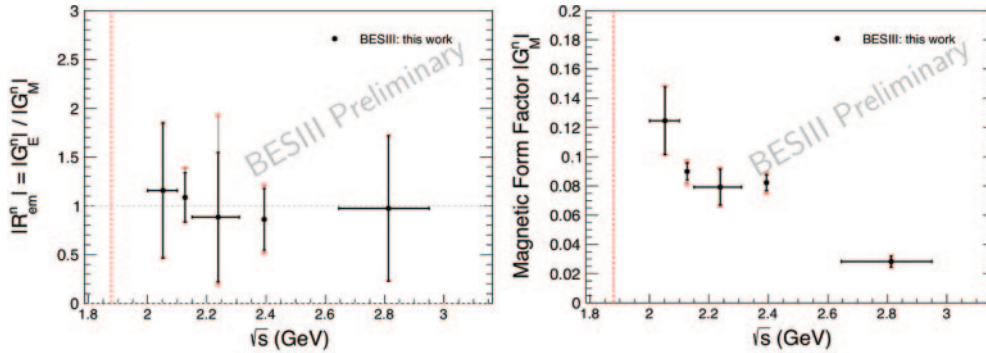
Fig. 5. – Results of the angular analysis to extract information of the neutron form factors. Vertical solid bars represents the statistical error, while the extended dashed bar with the arrow represents the systematic contribution. Horizontal bars represents the energy interval considered to extract the central value. (a) Ratio between the electric and the magnetic form factor. (b) First direct measurements of the magnetic form factors.
