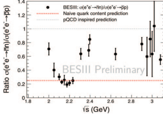
Fig. 4. – Ratio between the \sigma(e^+e^- \rightarrow n\bar{n}) and \sigma(e^+e^- \rightarrow p\bar{p}) cross sections using all recent BESIII data. Two theoretical predictions are also showed to magnify the different behaviour in the two energy regions.
