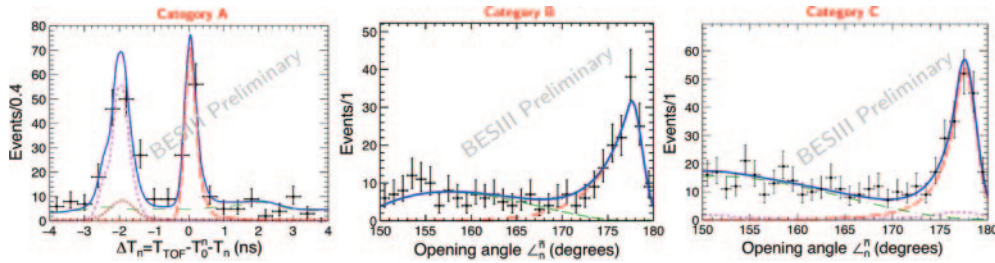
Fig. 2. – Results from the fit to the data at 2.396 GeV. Data are shown as points with error bars. Solid lines represent the total fit, dashed lines are the signal component, while dotted ones are from the background contributions.
