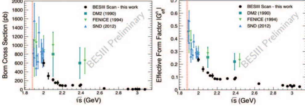
Fig. 3. – Comparison of the results of this work with other recent results. Black dots are the results of this work, squares represents the results from ref. [1], pointing down triangles are from ref. [2], and pointing up triangles are from refs. [3,4]. Left: Born cross section. Right: effective form factor.
