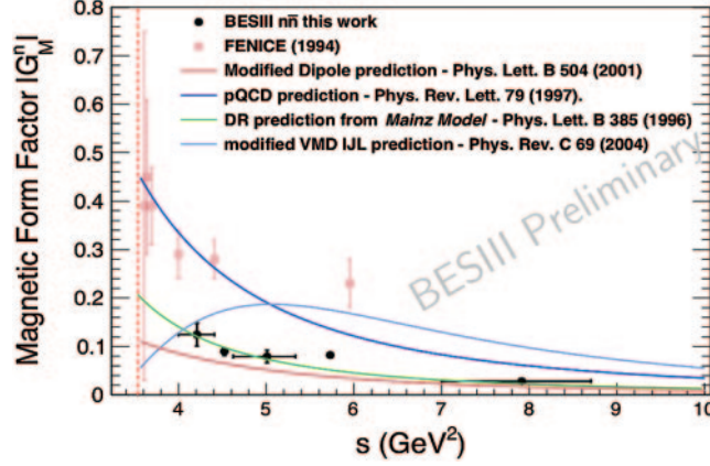
Fig. 6. – Comparison between the available measurements of the magnetic form factor and different theoretical models. Black dots are from this work, while squares are from ref. [2].
