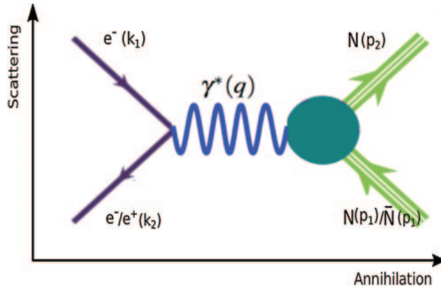
Fig. 1. – Sketch of the annihilation process at e^+e^- factories.
