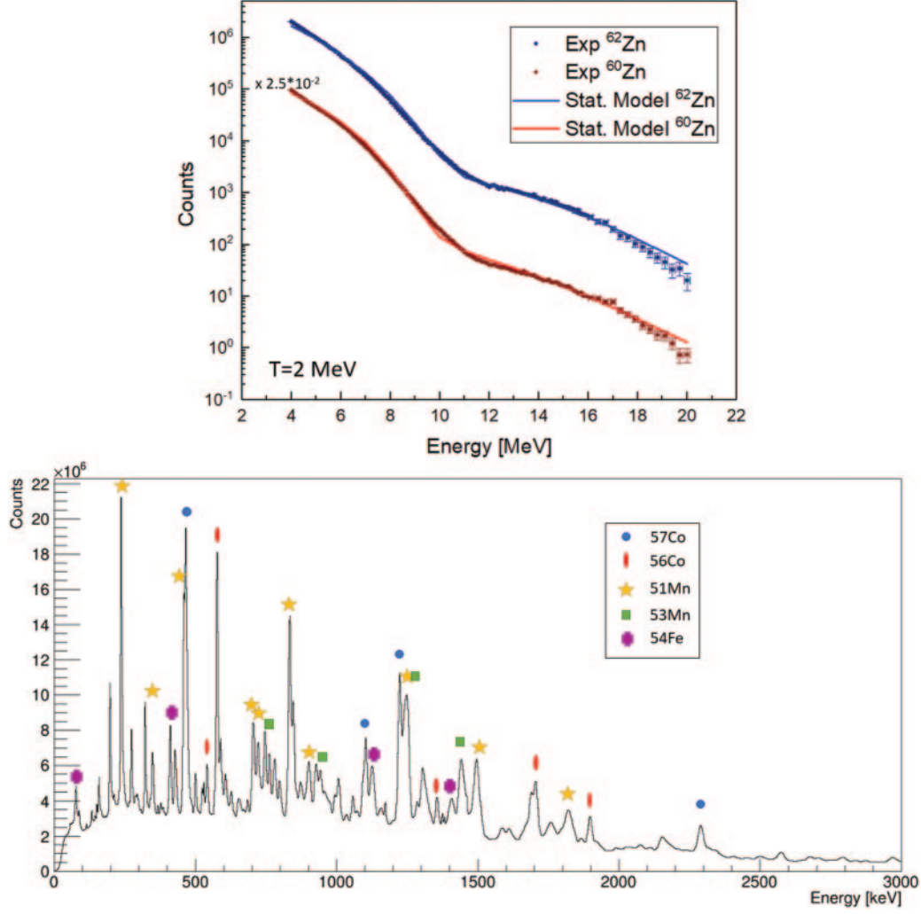
Fig. 1. – Upper part: Experimental spectra for ^{62}\text{Zn} (blue points) and ^{60}\text{Zn} (red points), together with the best fits with the statistical model for ^{62}\text{Zn} (blue line) and ^{60}\text{Zn} (red line). Lower part: HPGe spectrum for the ^{32}\text{S} + ^{28}\text{Si} \rightarrow ^{60}\text{Zn}^* reaction at T = 2.4 MeV. Transitions belonging to the main residual nuclei produced during the compound nucleus decay ( i.e. , ^{57}\text{Co} , ^{56}\text{Co} , ^{51}\text{Mn} , ^{53}\text{Mn} , ^{54}\text{Fe} ) are indicated with different symbols.
