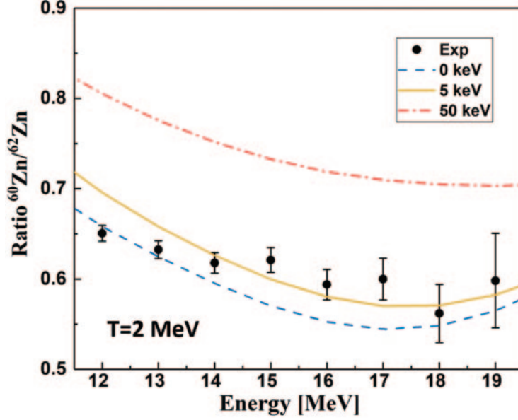
Fig. 2. – Experimental ratio (points) of ^{60}\text{Zn}/^{62}\text{Zn} for T = 2 MeV, together with the statistical model (CASCADE) ratios corresponding to different Coulomb spreading width values (lines). The blue dashed line and the red dot-dashed line are, respectively, the ratios with \Gamma^\downarrow = 0 keV and \Gamma^\downarrow = 50 keV (the maximum possible value). The yellow line is, instead, the ratio with \Gamma^\downarrow = 5 keV (for T = 2 MeV). The result of the minimization of the \chi^2 is, indeed, \Gamma^\downarrow = 5 \pm 3 keV, for the lower temperature, and \Gamma^\downarrow = 7 \pm 3 keV, for the higher temperature.
