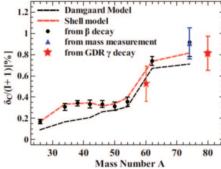
Fig. 5. – The isospin-mixing correction \delta_c , as a function of the nuclear mass number A , is shown. The dashed black and red lines are, respectively, the Damgaard model [34] and the shell model [35] predictions. The red star at mass 80 is the value obtained in [29], whilst the red star at mass 60 is the value of \delta_c extracted in this work. Black circles and the blue triangle are the experimental points extracted from the \beta -decay [1] and from the mass measurement [32], respectively.
