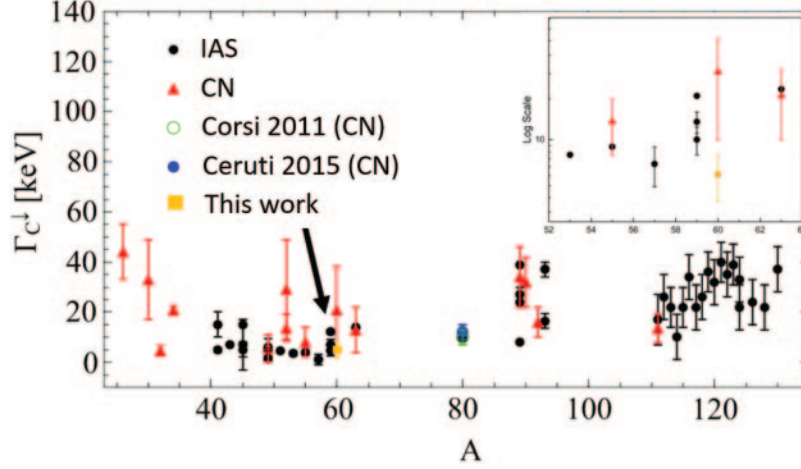
Fig. 3. – Values of the Coulomb spreading width obtained in the IAS (black dots) and in the CN (red triangle) [27,28]. The blue and green points are the values obtained in [29] and [15], while the orange square is the value obtained in this work. At the top right corner, there is a log scale zoom in the region of the obtained point.
