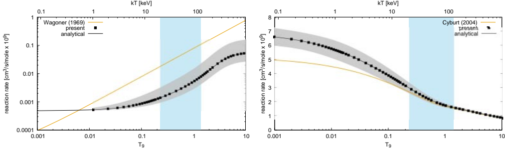
Fig. 1. – Reaction rates N_A\langle\sigma v\rangle for the {}^7\text{Be}(n, \alpha){}^4\text{He} (left) and {}^7\text{Be}(n, p){}^7\text{Li} (right), shown in comparison to rates evaluated before the n_TOF measurements. The gray bands around the analytical curves indicate the evaluated uncertainties on the rates, while the vertical band indicates the temperature of interest in BBN network calculations.
