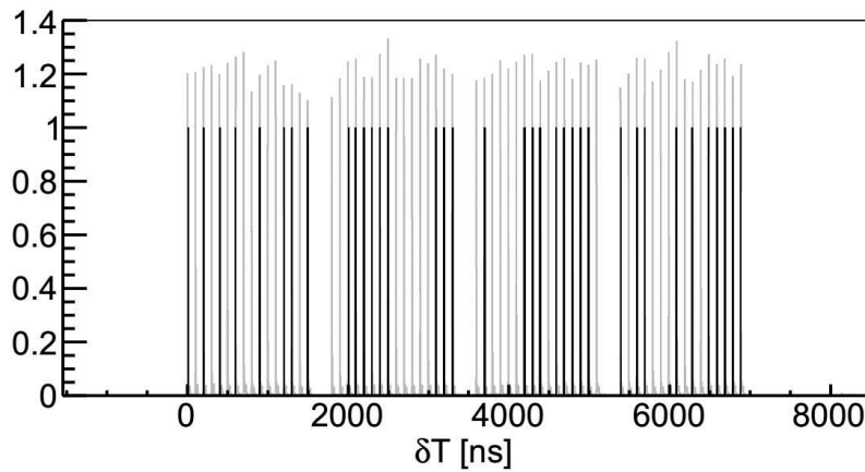
Fig. 1. – Comparison of the \delta T values of the 48 selected events (black lines) with the summed waveforms of proton extraction (grey lines). The origin of time for the waveforms is given by the maximum of the first bunch.
